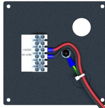
Figure 5-7 9SE DFB Wiring
