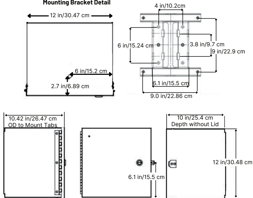
T-Series Controllers Mounting Bracket Detail
