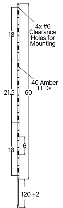
Sign Post Flashers with Amber LEDs
