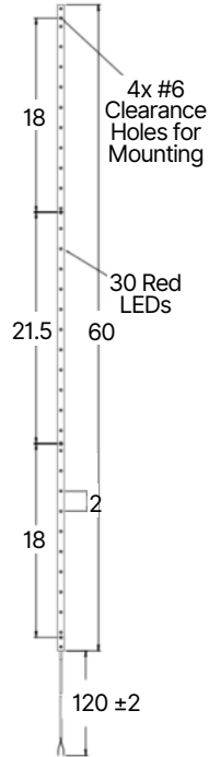
Sign Post Flashers with Red LEDs
