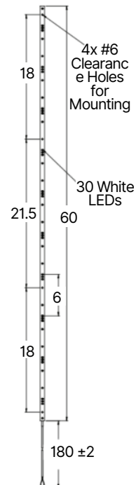
Sign Post Flashers with White LEDs
