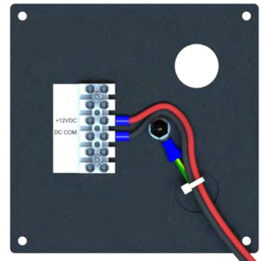
Figure 5-7 9SE DFB Wiring
