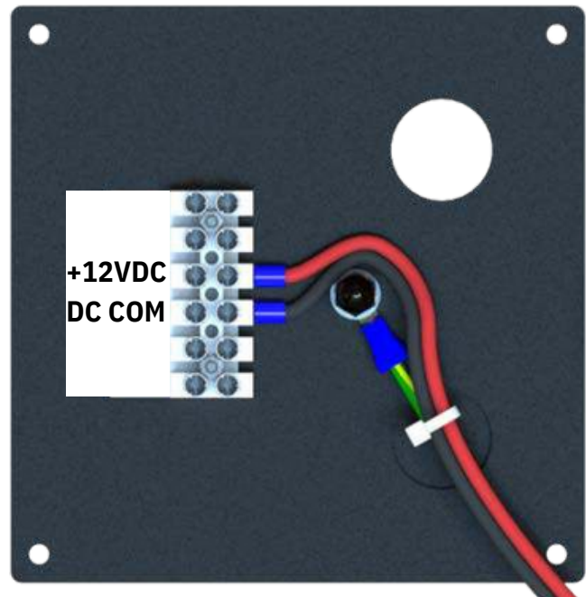
Figure 5-7 9SE DFB Wiring
