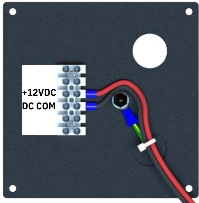
Figure 5-7 9SE DFB Wiring
